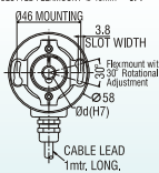
MODEL J-260-ND-SL DOUBLE SIDE SLOTTED FLEXMOUNT Ø46mm = SF1
