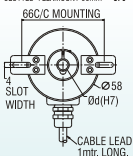
MODEL J-260-ND-SL DOUBLE SIDE SLOTTED FLEXMOUNT Ø66mm = SF3
