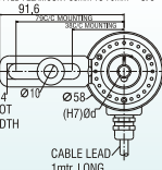
MODEL J-260-ND-SL SINGLE SIDE SLOTTED FLEXMOUNT Ø38mm TO 79mm = SF5
